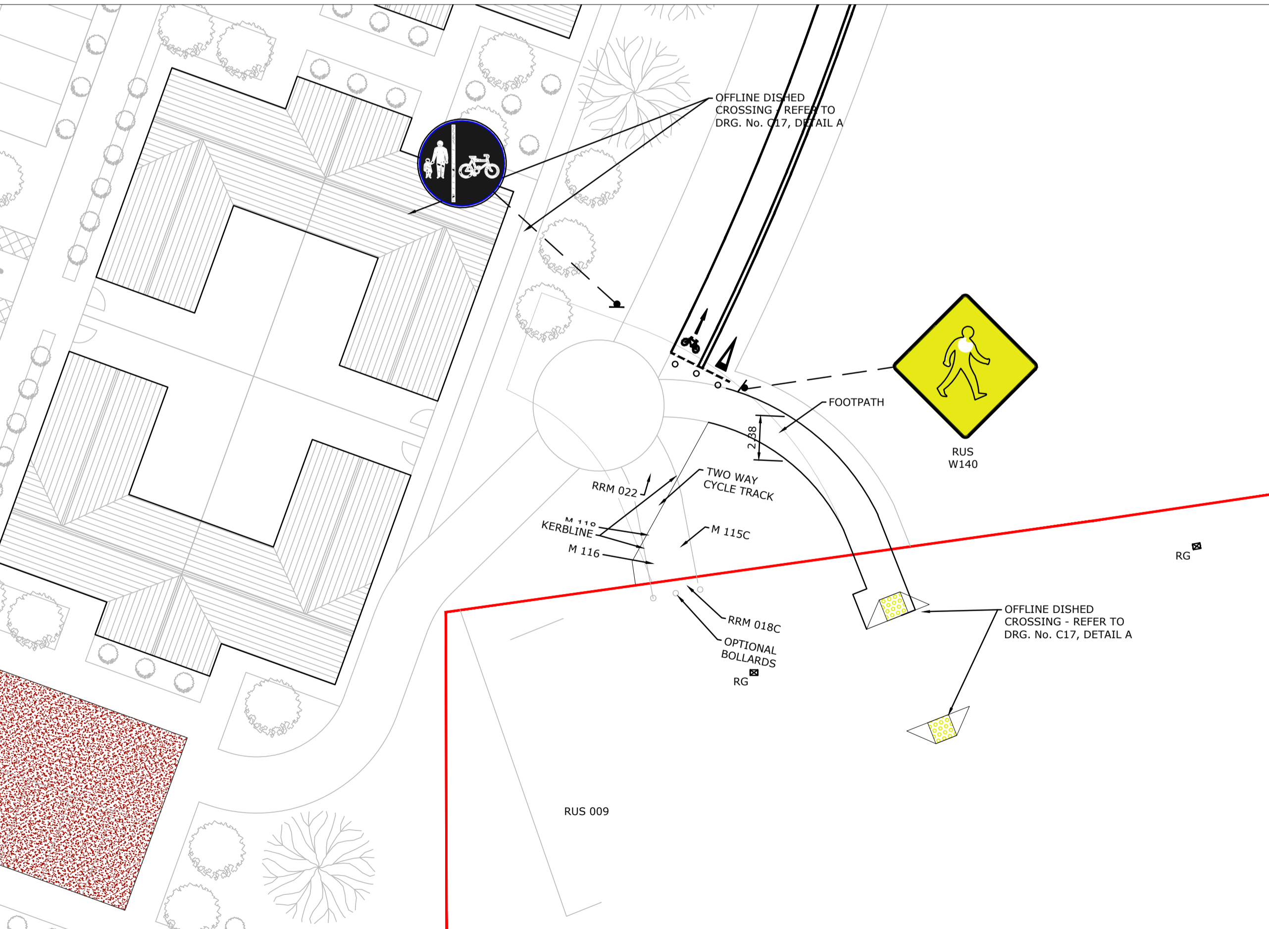
B PLAN: CYCLE TRACK TO NEIGHBOURING ESTATE C13 Scale 1:200
