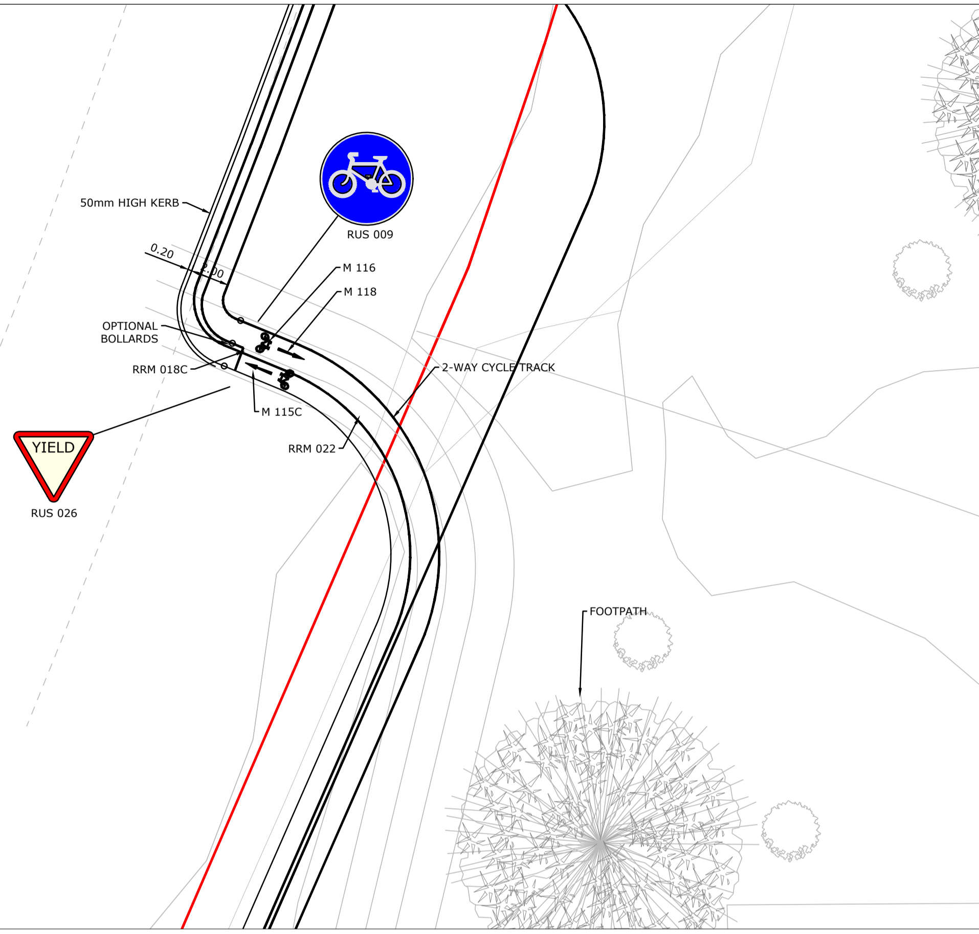
A PLAN: CYCLE TRACK TO R510 C13 Scale 1:200
